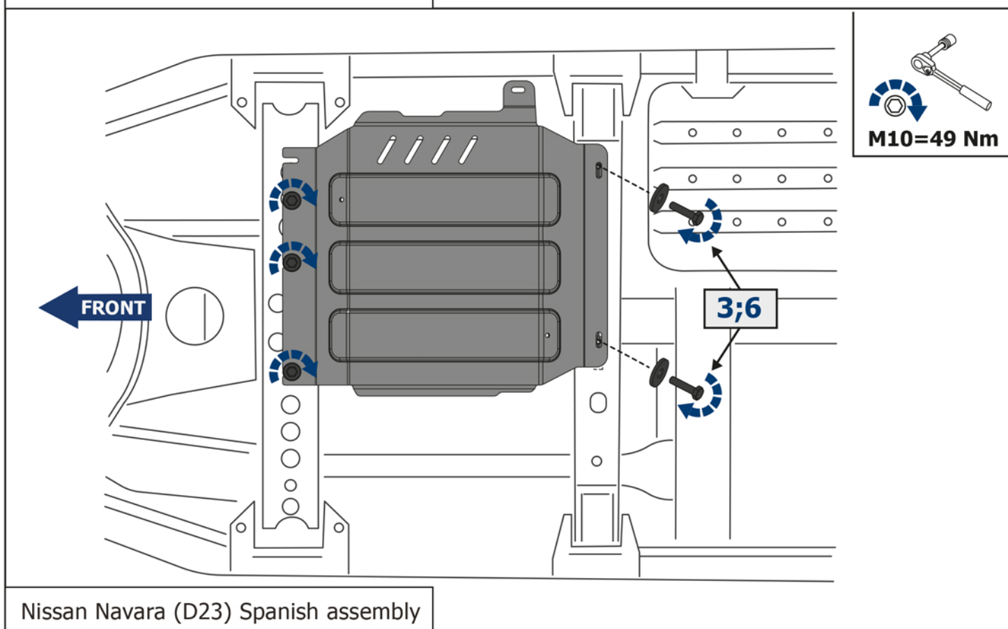
Nissan Navara (D23) Spanish assembly
