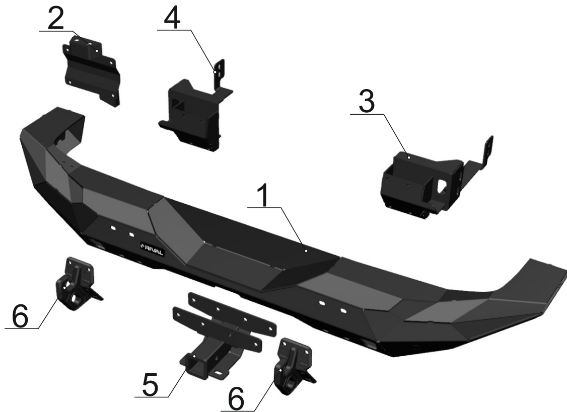
Rear full width bumper 2D.2723.1-NL
