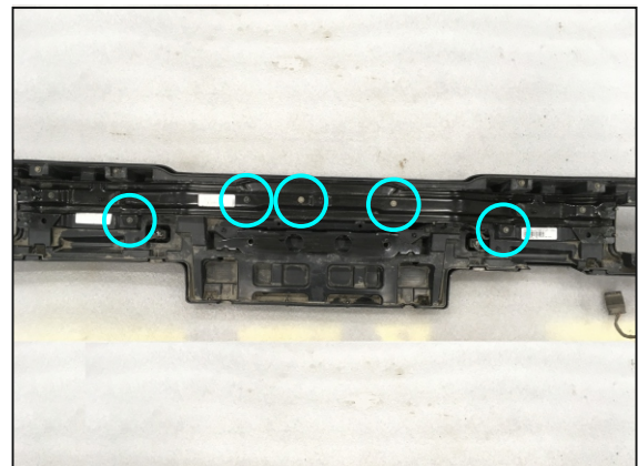
24. Unscrew 5 screws that hold bumper reinforcement.
