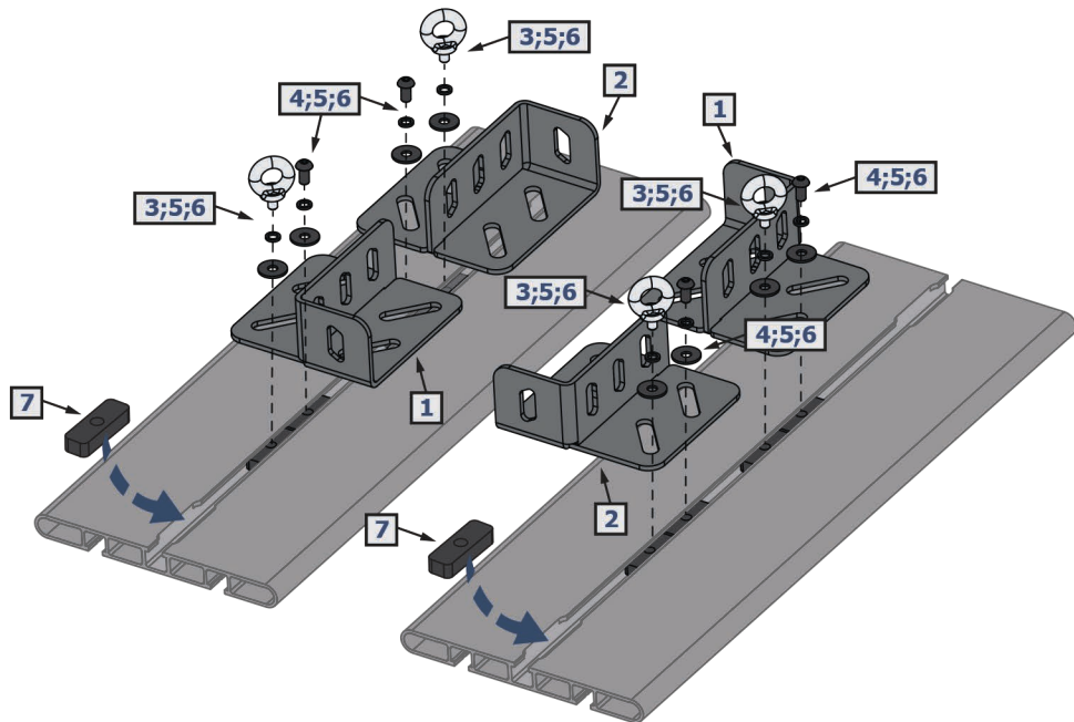
UNIVERSAL RACK CARGO HOLDERS FOR RIVAL MODULAR RACK 2MD.0003.1
