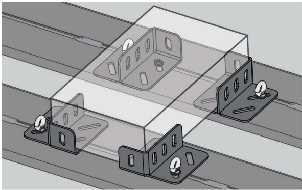
UNIVERSAL RACK CARGO HOLDERS FOR RIVAL MODULAR RACK 2MD.0003.1
