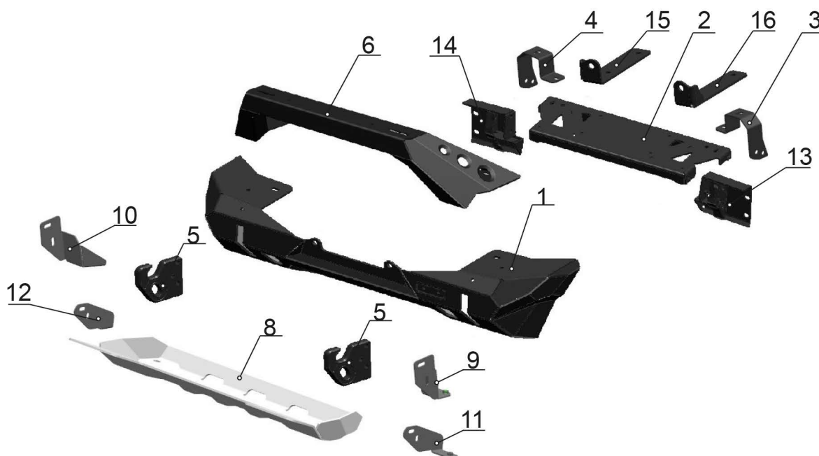
Front stubby bumper 2D.2702.2-NL
