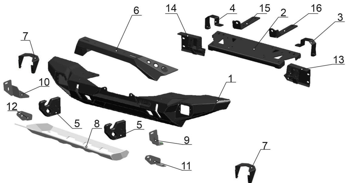
Front full width bumper 2D.2701.2-NL
