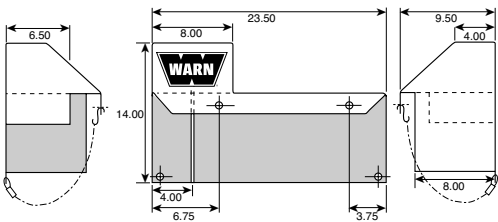
PN 13918 Fits 9.5xp, XD9000, M8000 and M6000 winches mounted on the Classic Bumper (when winch control pack is mounted behind the motor)
