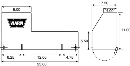
PN 13916 For the 9.5xp, XD9000, M8000, VR8000, VR10000, VR12000 and M6000 winches, mounted the Trans4mer and Combo Kit
