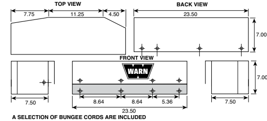
PN 18250 Fits 9.5ti and XD9000i mounted on the Classic Bumper
