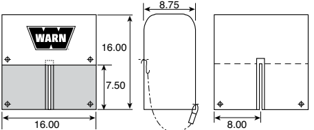
PN 8557 Fits the M8274-50 winch
