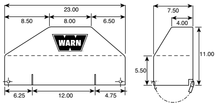
PN 13917 Fits 9.5cti, 9.5ti, XD9000i, and winches mounted on the Trans4mer, Combo Kit, Multi-Mount and Flatbed Mount
